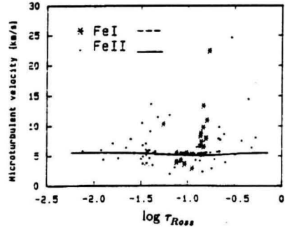
Figure 4: averaged \zeta_{\mu} for FeI and FeII for the model with T_{eff} = 10200 K against Rosseland mean optical depth.
