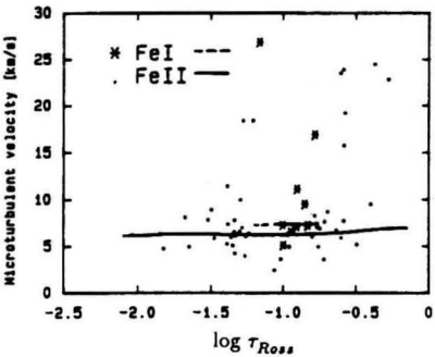
Figure 3: averaged \zeta_{\mu} for FeI and FeII for the model with T_{eff} = 10300 K against Rosseland mean optical depth.
