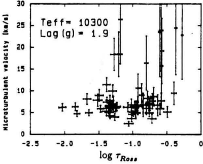
Figure 2: \zeta_{\mu} against Rosseland mean optical depth for the Kurucz model with T_{eff} = 10300 and \log g = 1.9 .
