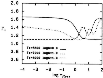
Figure 2: \Gamma_1 throughout the Kurucz model atmospheres of extreme supergiants with T_{\text{eff}} = 5500, 7000 and 8000 \text{ K} .
