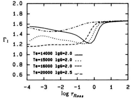
Figure 4: \Gamma_1 throughout the Kurucz model atmospheres with T_{\text{eff}} between 14000 K and 20000 K.
