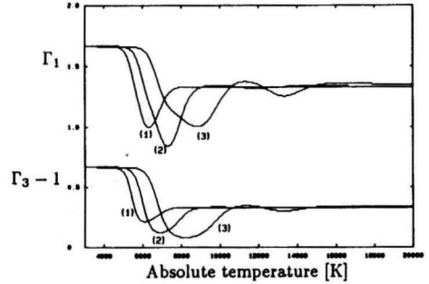
Figure 1: \Gamma_1 and \Gamma_3 - 1 for a system with ionization and radiation with electronpressure (1) P_e=0.1 , (2) P_e=1.0 , (3) P_e=20.0
