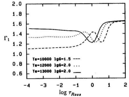
Figure 3: \Gamma_1 throughout the Kurucz model atmospheres with T_{\text{eff}} = 10000 \text{ K}, 12000 \text{ K}, 13000 \text{ K} .
