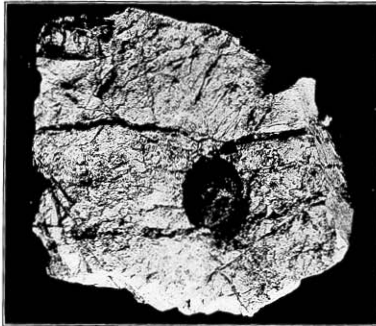
Fig. 1. Manganese nodule in jurassic marl with chert-nodules and radiolaria from Sua Lain, Island of Rotti. Original size.
