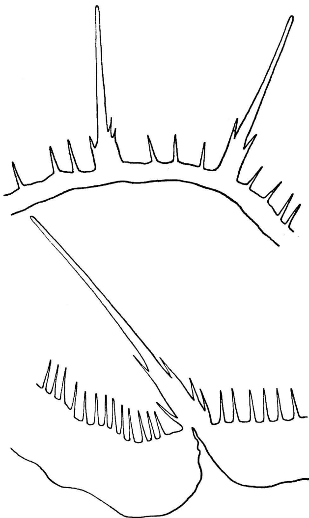
Fig. 5. Loxothylacus variabilis , specimen on Actaea hirsutissima , section of the two layers of external cuticle. \times 530 .
