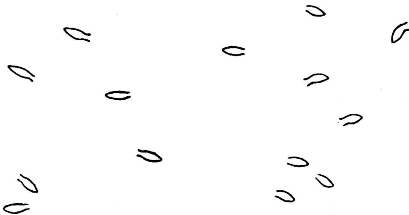
Fig. 4. Sacculina ignorata , retinacula as they are arranged on the internal cuticle. \times 530 .
